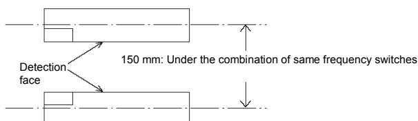
(2) Faced arrangement
