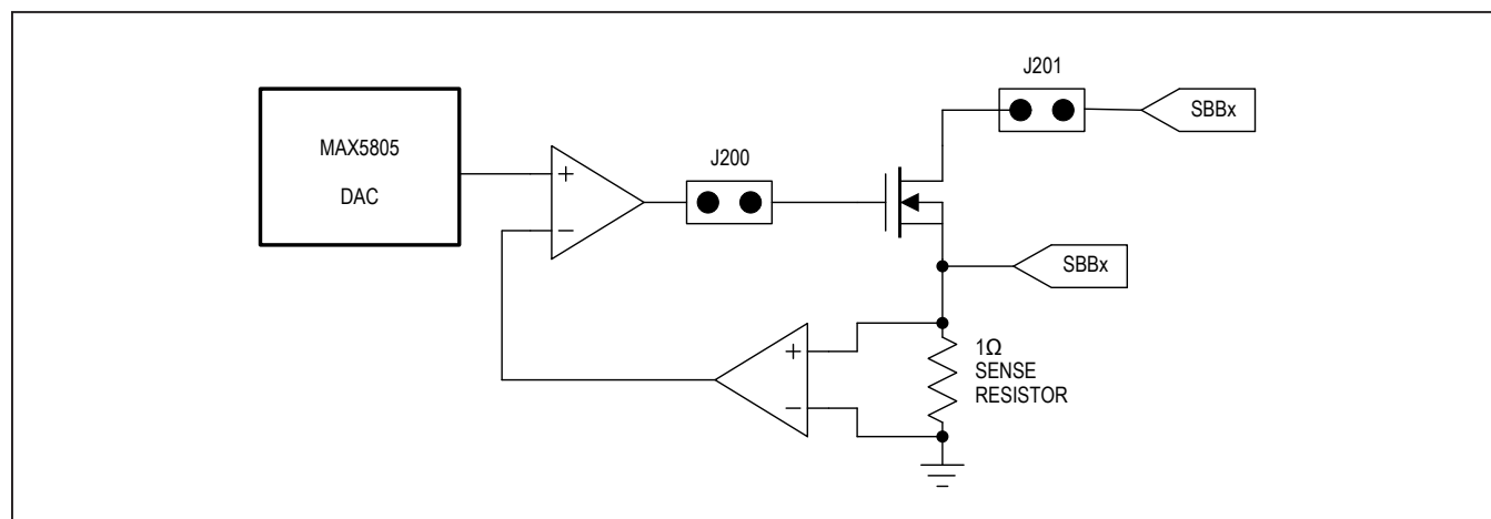
Figure 5. Electronic Load Circuit
