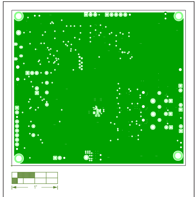
MAX77680/MAX77681 EV Kit PCB Layout—Internal Layer 2
