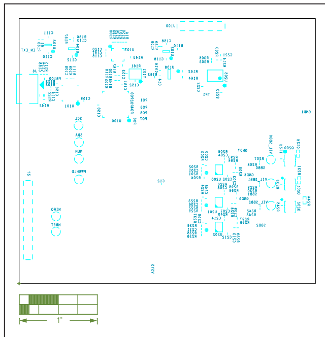
MAX77680/MAX77681 EV Kit Component Placement Guide— Bottom Silkscreen
