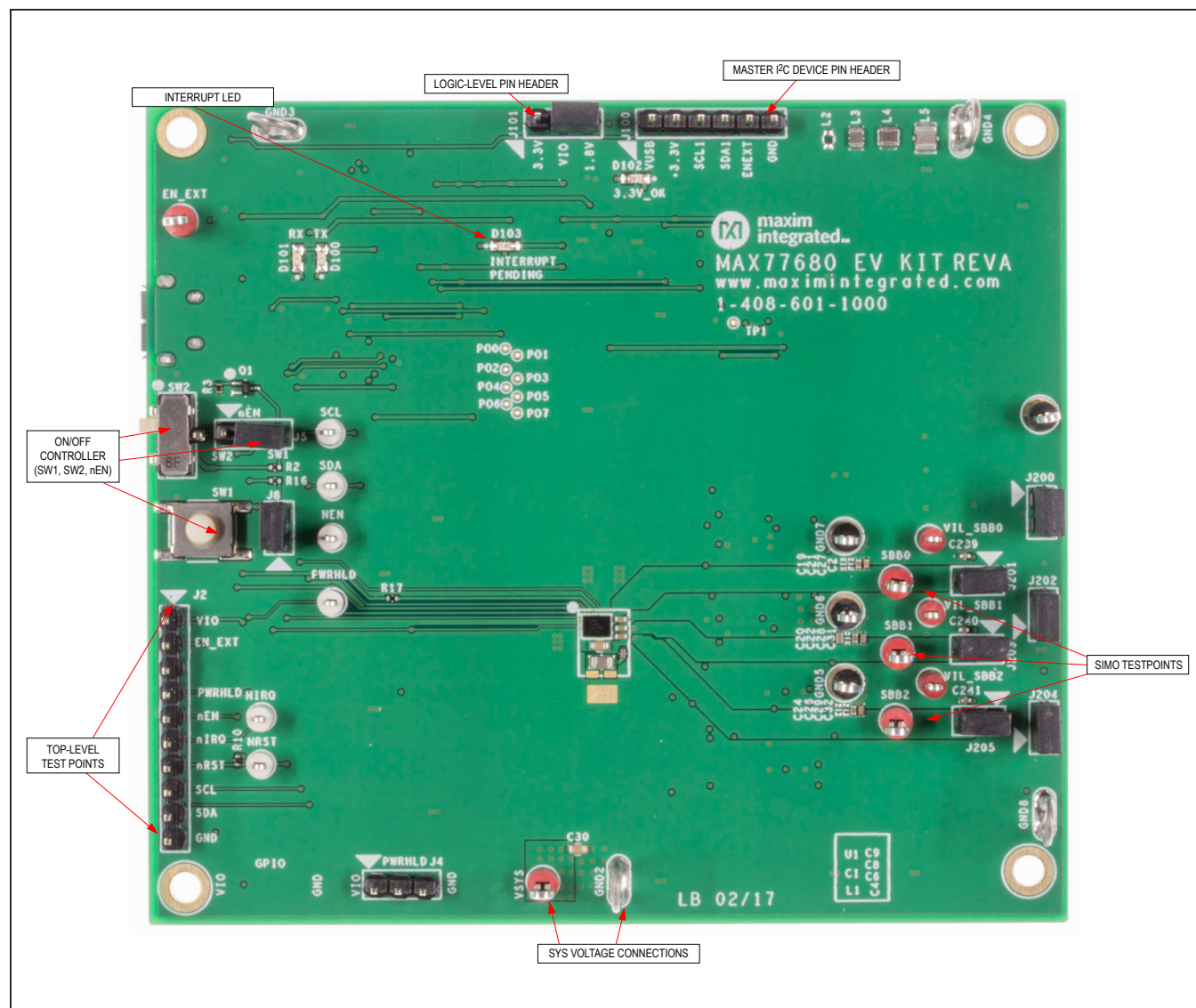
Figure 3. MAX77680/MAX77681 EV Kit Top View
