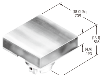
AT3027 Square Solid Cap for Nonilluminated ABS Resin & Brushed Chrome Plating Color: P (Brushed Chrome) Series: YB2
