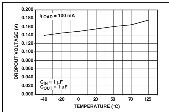
FIGURE 2-2: Dropout Voltage vs. Temperature ( I_{LOAD} = 100 mA ).
