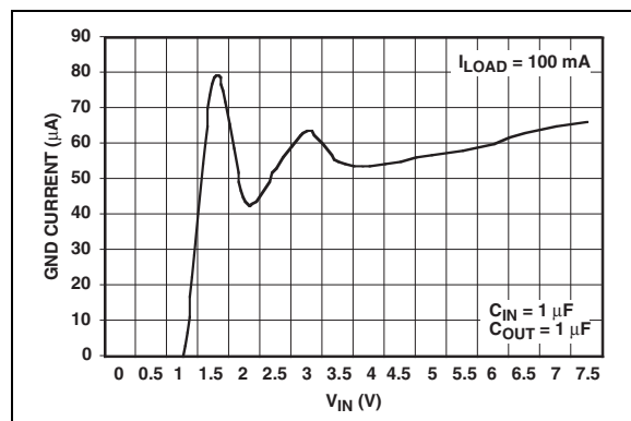
FIGURE 2-6: Ground Current vs. V_{IN} ( I_{LOAD} = 100 mA ).
