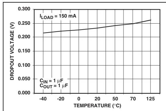
FIGURE 2-5: Dropout Voltage vs. Temperature ( I_{LOAD} = 150 mA ).
