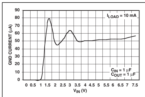
FIGURE 2-3: Ground Current vs. V_{IN} ( I_{LOAD} = 10 mA ).
