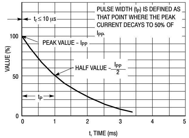
Figure 2. Pulse Waveform
