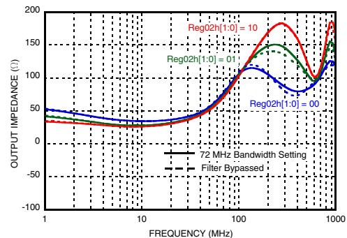
Figure 30. Output Impedance
