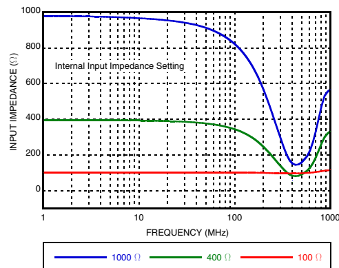
Figure 29. Input Impedance
