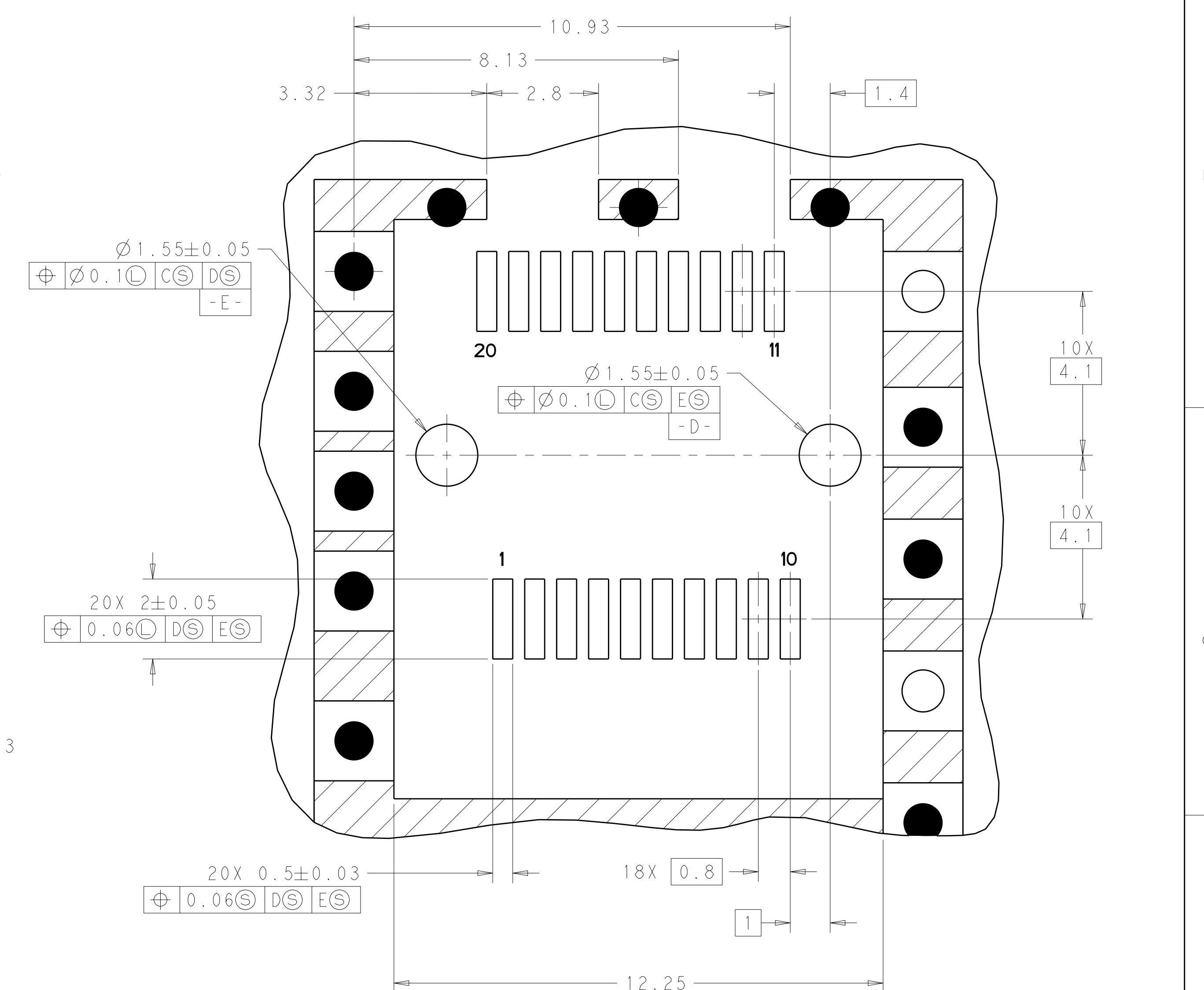
DETAIL J RECOMMENDED PT CONNECTOR LAYOUT SCALE 12:1
