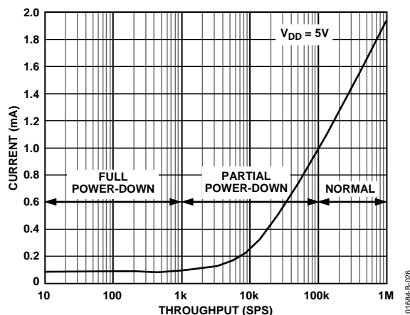
Figure 25. Typical AD7495 Current vs. Throughput
