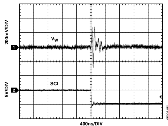
Figure 29. Digital Feedthrough
