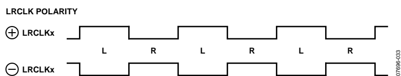
Figure 32. Serial Input LRCLK Polarity
