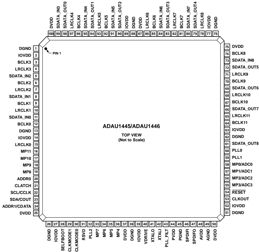
Figure 7. Pin Configuration
