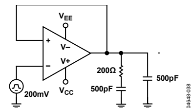
Figure 38. Snubber Network
