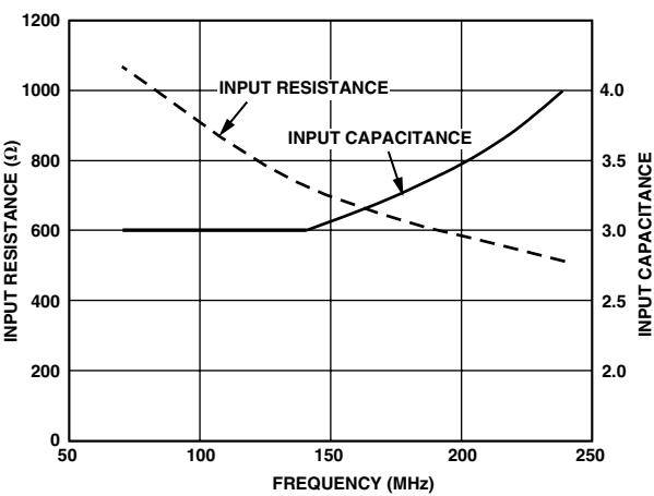
TPC 15. Input Impedance vs. Frequency, Z_{IN} = R \parallel C
