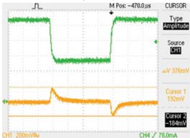
Stepload Transient Response (Vin = 24V, Iout = 50% to 75%, Cload = 1μF || 10μF, Ta = +25°C) CH1 = Vout, CH4 = Iout
