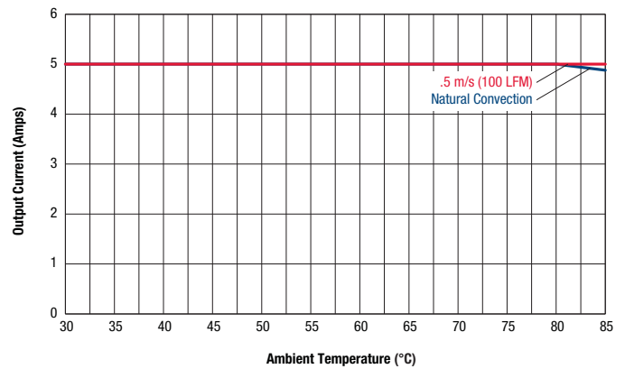
Maximum Current Temperature Derating at sea level Vin 75 (air flow from Pin J1 to Pin J3 on PCB)
