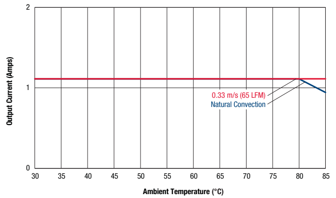
Maximum Current Temperature Derating at sea level Vin = 36V (air flow is from J1 to J3 on PCB)*
