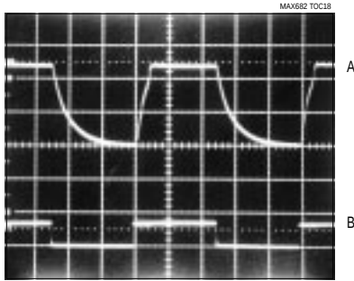
SHUTDOWN TIMING
