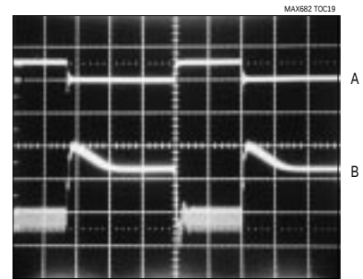
LOAD-TRANSIENT RESPONSE
