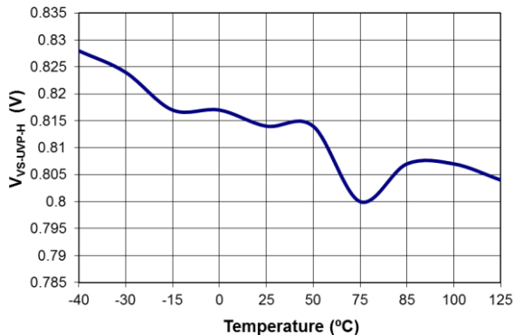
Figure 17. Output Under-Voltage Protection ( V_{VS-UVP-H} ) vs. Temperature
