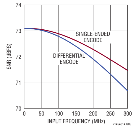
LTC2145-14: SNR vs Input Frequency, -1\text{dBFS} , 125\text{Mps} , 2\text{V} Range
