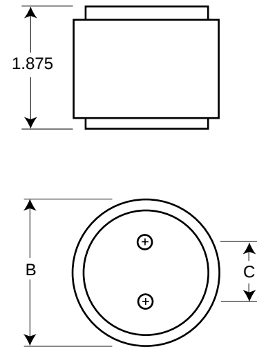
Fig. 1: 1000-3000 Amp Range
