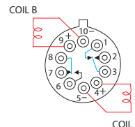
SCHMATIC (Coil A Last Energized) 422H
