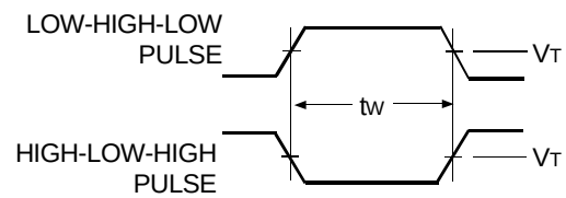
Pulse Width
