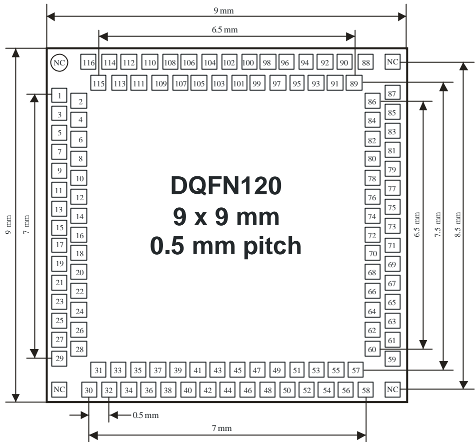
Figure 18: DQFN120 package (top view)
