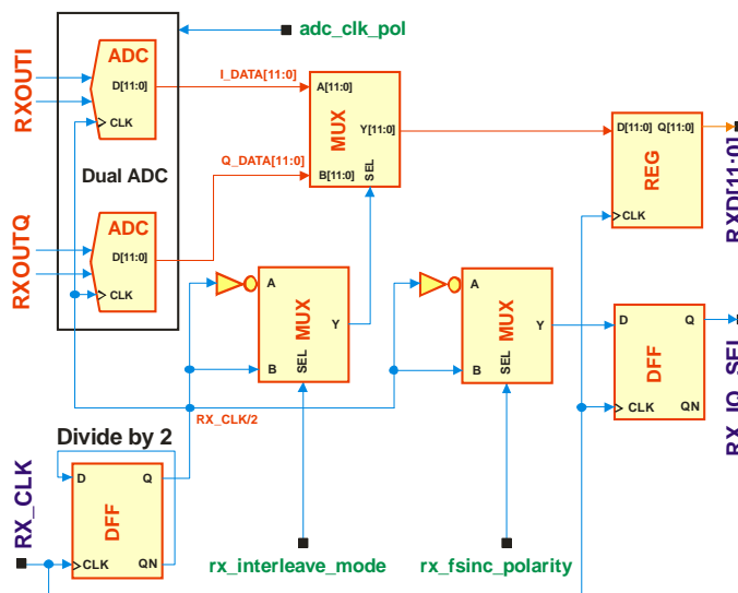
Figure 11: RX data interface
