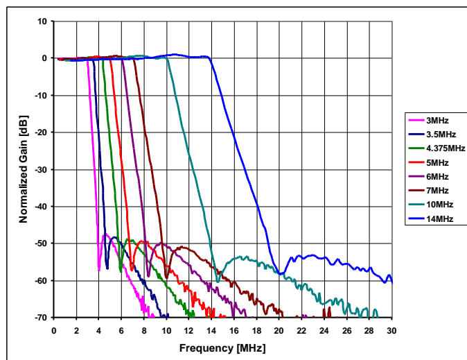
Figure 6: Measured TX/RX LPF amplitude responses
