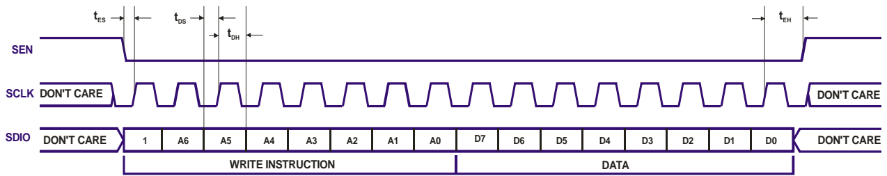
Figure 14: SPI write cycle, 3-wire and 4-wire modes
