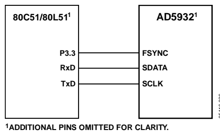
Figure 36. 80C51/80L51 to AD5932 Interface
