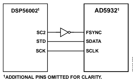
Figure 37. DSP56002 to AD5932 Interface
