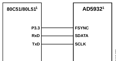
Figure 36. 80C51/80L51 to AD5932 Interface
