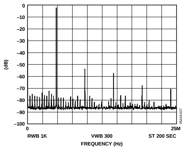
Figure 27. f_{MCLK} = 50 MHz, f_{OUT} = 4.8 MHz, Frequency Word = 189374
