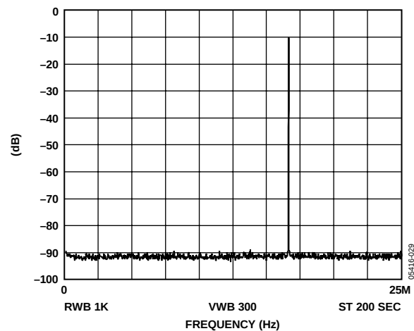
Figure 29. f_{MCLK} = 50 MHz, f_{OUT} = 16.667 MHz = f_{MCLK}/3 , Frequency Word = 555555
