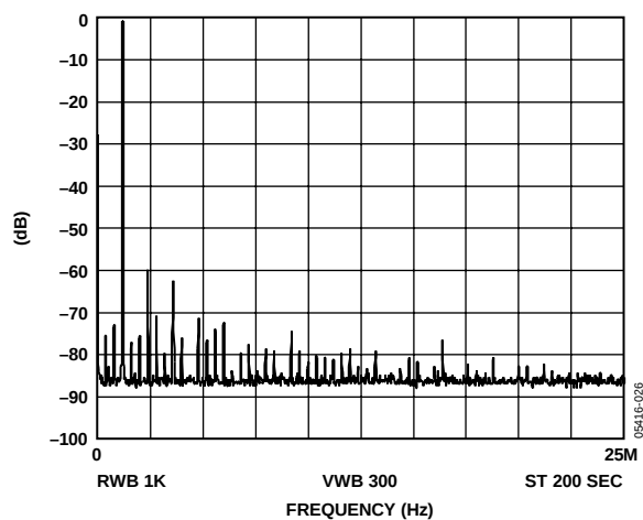
Figure 26. f_{MCLK} = 50 MHz, f_{OUT} = 1.2 MHz, Frequency Word = 0624DD
