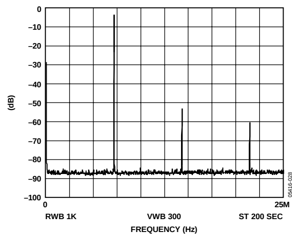
Figure 28. f_{MCLK} = 50 MHz, f_{OUT} = 7.143 MHz = f_{MCLK}/7 , Frequency Word = 249249
