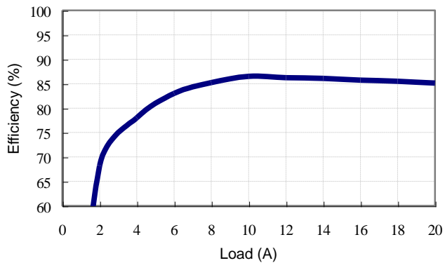
Figure 5: Converter efficiency vs. output current (1.2V output voltage, 12V input)
