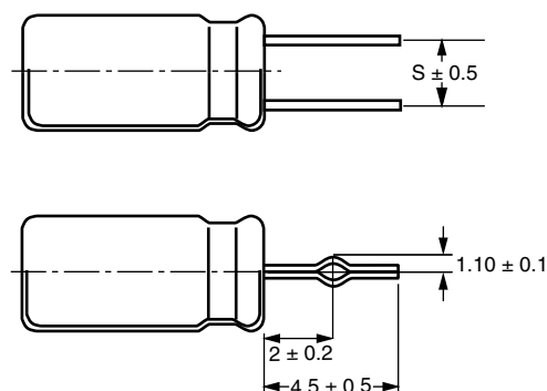
10 \leq \varnothing D \leq 18 leads shortened and formed MALREKE06... (S = 5/7.5 mm)
