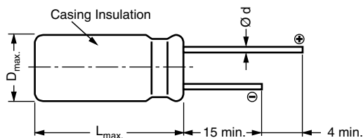
\varnothing D \leq 18 long leads MALREKE00...
