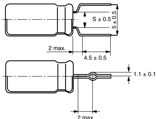
\varnothing D \leq 8 leads shortened and formed MALREKE09... (S = 2.0/2.5/3.5 mm)
