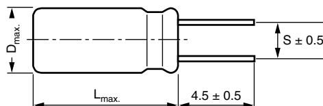
\varnothing D \leq 18 shortened leads MALREKE05... (S = 2/2.5/3.5/5/7.5 mm)
