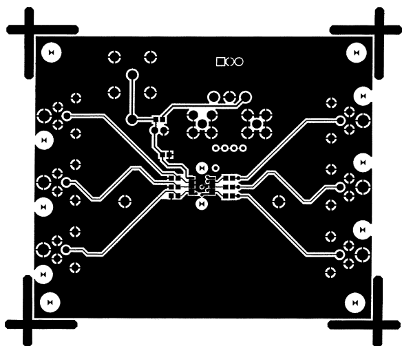
Figure 6. Component Side
