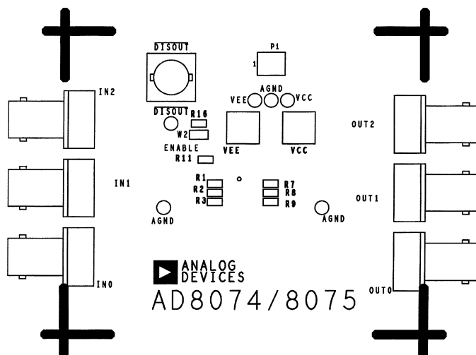
Figure 8. Silkscreen Top
