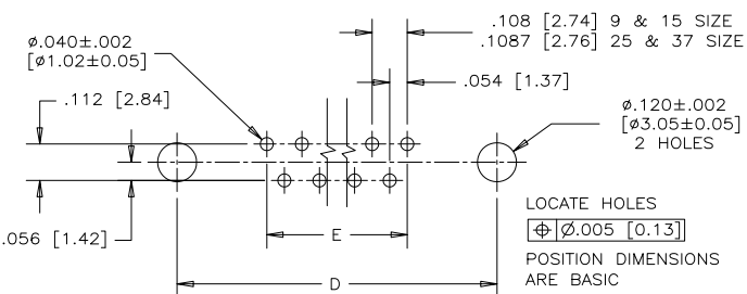
RECOMMENDED P.C.B. LAYOUT (COMPONENT SIDE OF BOARD)
