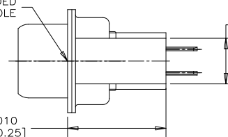
END VIEW
