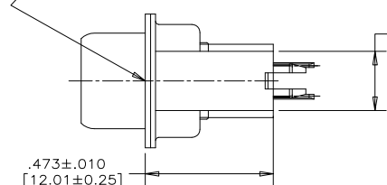
END VIEW
