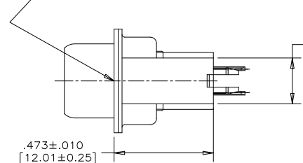
END VIEW
