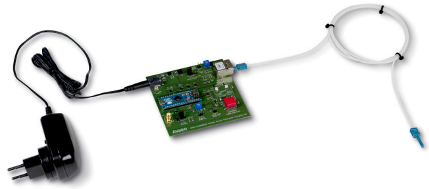
Figure 5. Configuration used to test the heartbeat loss alarm of the evaluation board
