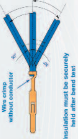
INSULATION CRIMP
