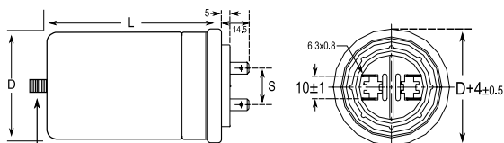
Threaded Mounting Stud D < 60: M6 x 12 D ≥ 60: M12 x 16
