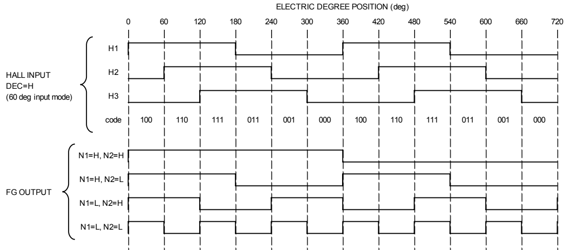
OUTPUT TIMING CHART 2 (60 deg Input Mode)
