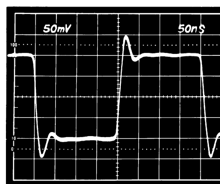
Figure 2b. AD849 Small Signal Pulse Response
