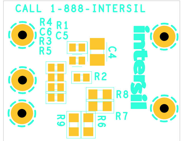
FIGURE 8. SILKSCREEN BOTTOM
