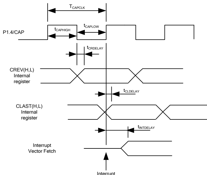
Figure 16. CAPTURE timing
