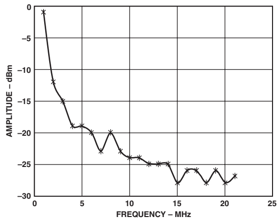
TPC 2. Input Sensitivity. V_{DD} = 3.3\text{ V} ; 100 pF on RF_{IN}
