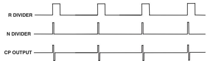
Figure 5. PFD Simplified Schematic and Timing (In Lock)
