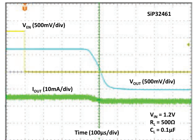
Fig. 37 - Turn-off Time
