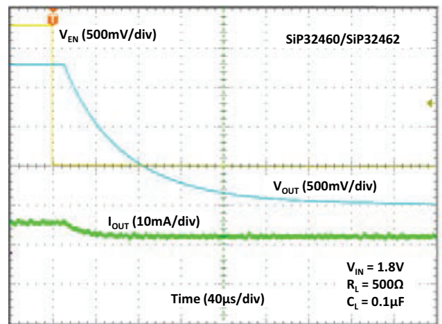
Fig. 36 - Turn-off Time
