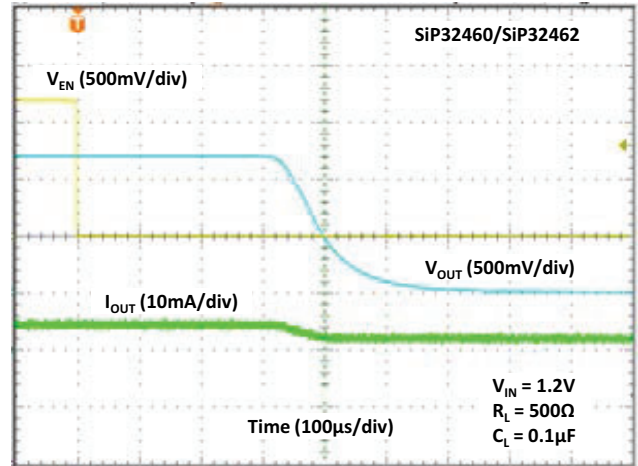
Fig. 35 - Turn-off Time
