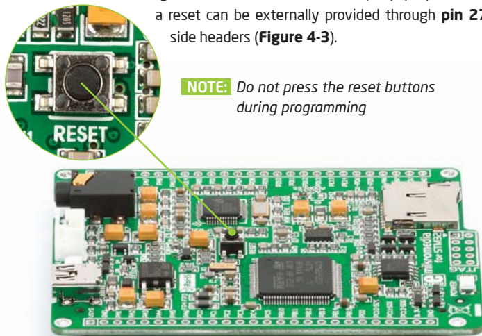
Figure 4-1: Reset button located at the backside of the board
