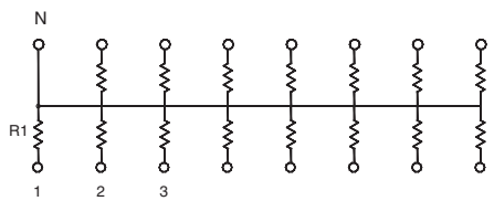
Schematic B Bussed
