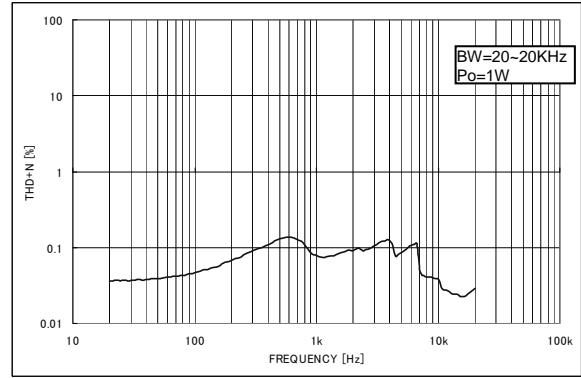
Fig.16 THD+N - Frequency
