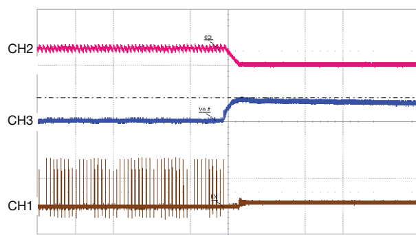
Fig. 14 - Load Step Overshoot Response, I_{OUT} = 3\text{ A} to 0\text{ A} CH2 (RED) = I_{COIL} (5 A/div), CH3 (BLU) = V_{OUT} (200 mV/div), CH1 (BRN) = LX (10 V/div), Time = 10 \mu\text{s}/\text{div}
