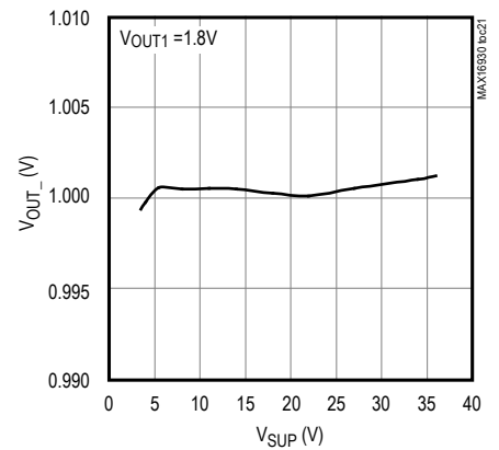
FB1 LINE REGULATION
