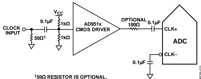
Figure 53. Single-Ended 1.8 V CMOS Input Clock (Up to 200 MHz)
