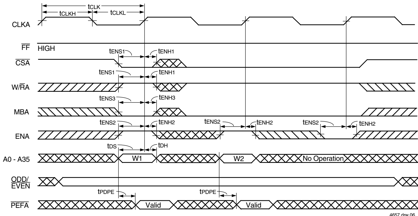
Figure 3. FIFO Write Cycle Timing
