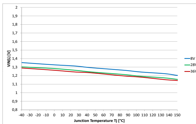
Figure 48 Input Voltage Threshold V_{IN(L)} = f(T_J; V_S)
