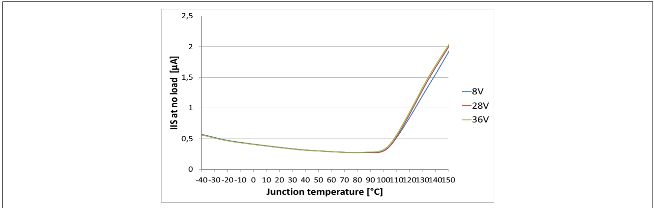
Figure 44 Current Sense at no Load I_S = f(T_J; V_S) , I_L = 0
