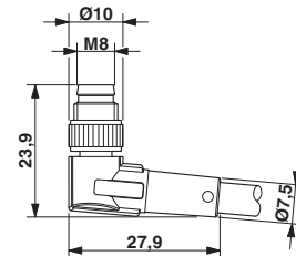
Plug M8 x 1, angled, shielded
