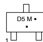
MSB92AS1WT1G
